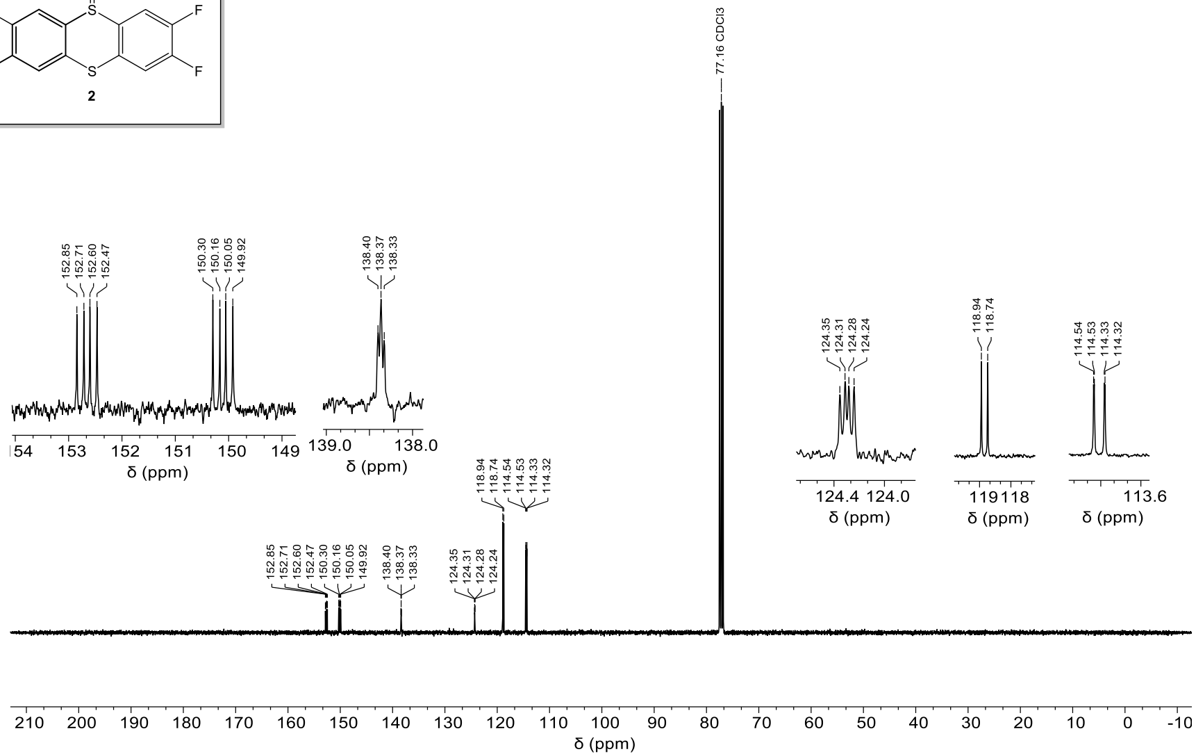
13 C NMR (101 MHz, CDCl 3 ) of 2,3,7,8-tetrafluorothianthrene-S-oxide (2).
